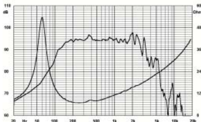
Frequency response ■ Box 20 dmc - 1W - 1m Impedance ■ (Iac=10mA)
